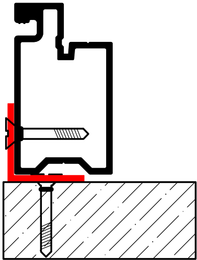
Angle Mount
