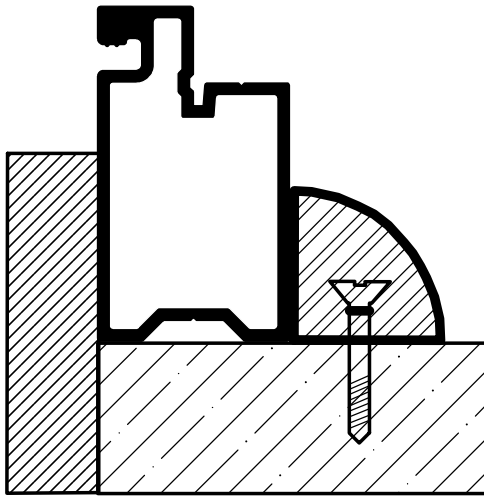
Large Stop w/t Trim Other Shapes May Be Used
