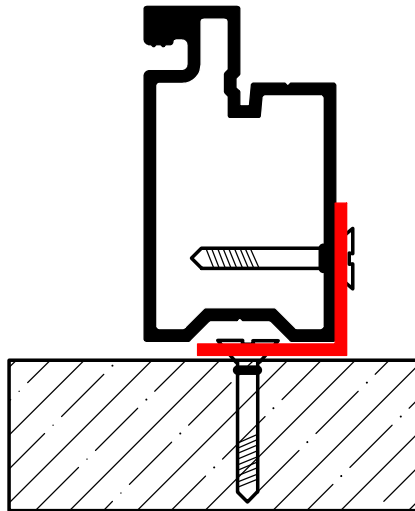
Angle Mount
