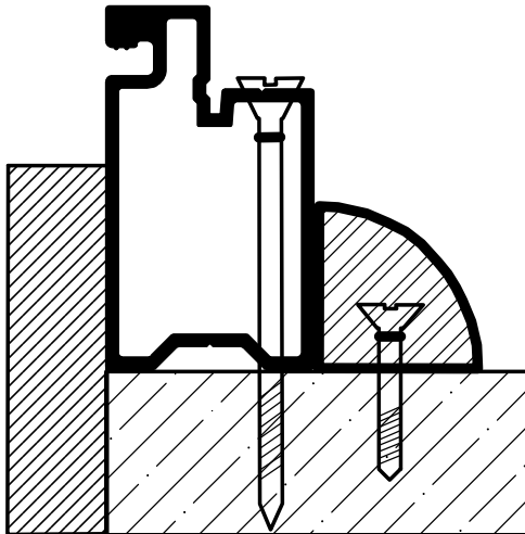
Large Stop w/t Trim (Side Screwed) Other Shapes May Be Used
