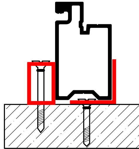
Reversed Angle Stop
