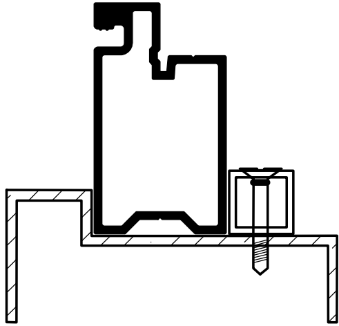
Store Front Extrusion
