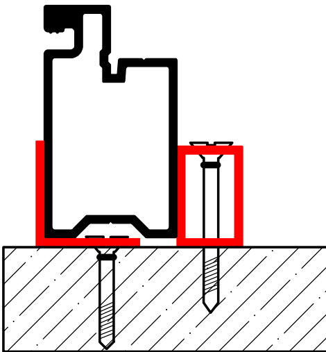
Angle Stop
