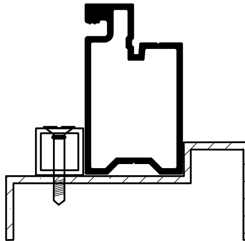
Store Front Extrusion
