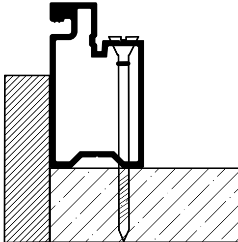
Large Stop (Side Screwed)
