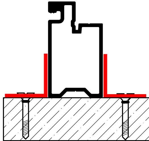
Double Angle
