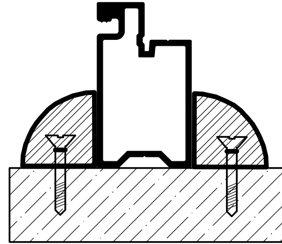
Small Stops Other Shapes May Be Used
