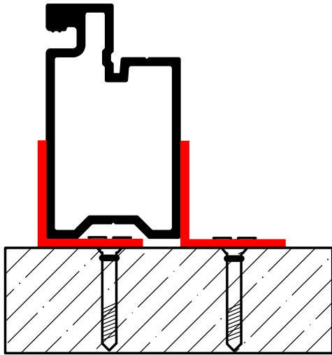
Double Angle
