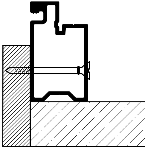
Large Stop Other Shapes May Be Used
