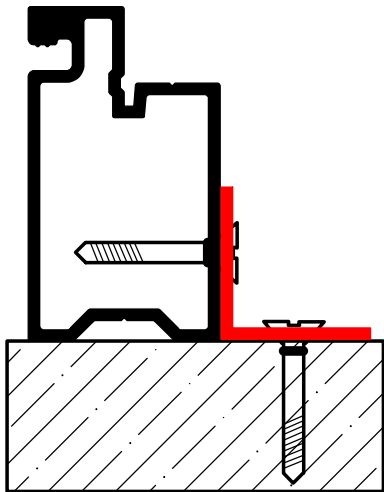
Angle Mount
