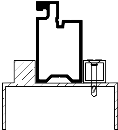
Store Front Extrusion
